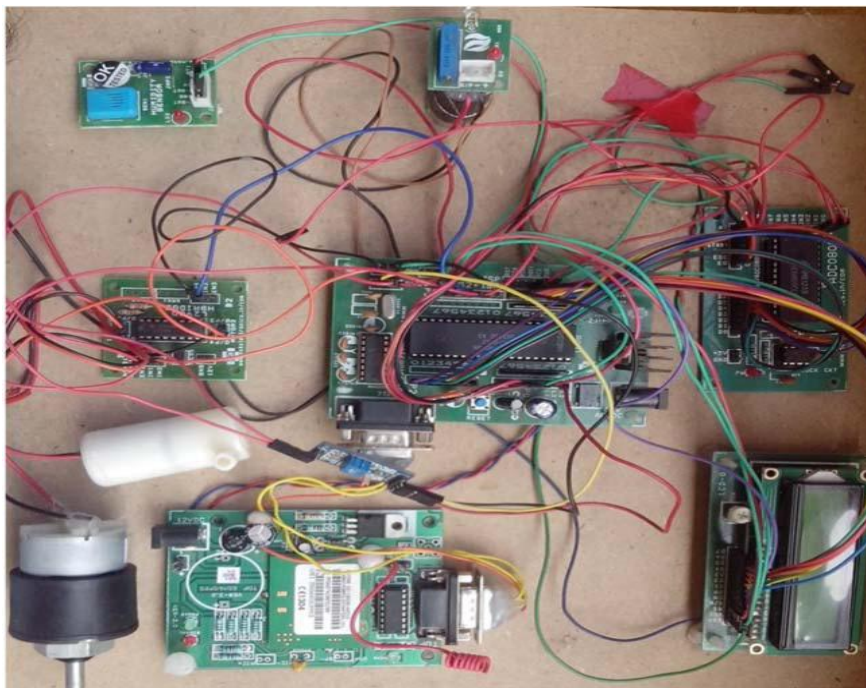
Fig 2. Model of the plant irrigation system
