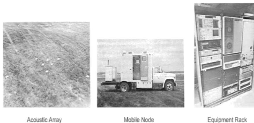
Fig.1. Components in the DSN test bed around 1985.
