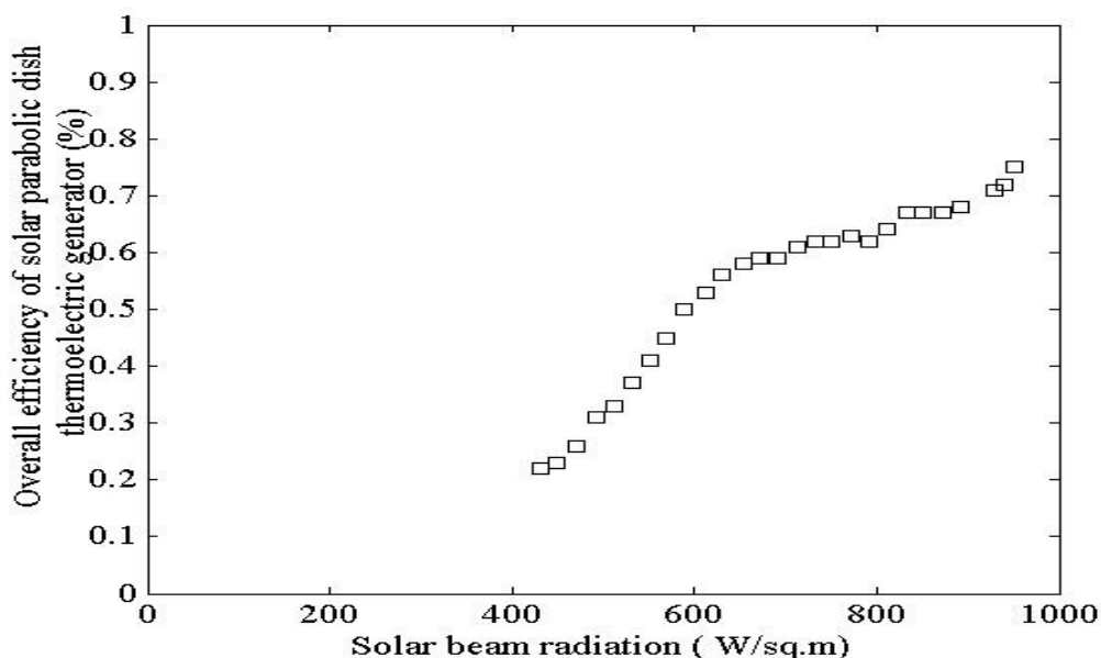
Figure 5: Overall efficiency of solar parabolic dish thermoelectric generator as function of solar beam radiation
