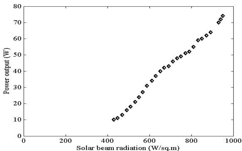
Figure 4: Maximum power output as function of solar beam radiation
