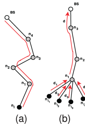
Fig.1. Provenance graphs for a sensor network.
