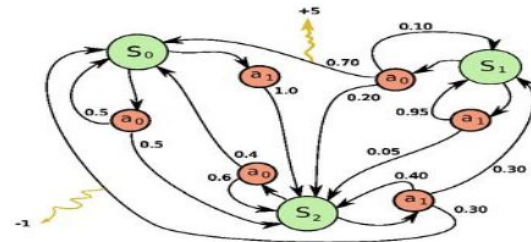
Fig 2.1: working procedure of Markov Decision Process
