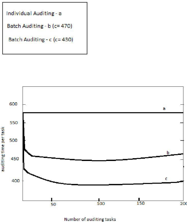
Fig.2 Comparison of auditing time between batch auditing and individual auditing.
