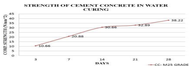
Fig. 2: The Compressive Strength of Cement Concrete with M25 Grade
