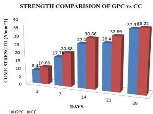
Fig. 3: Strength Comparison of Geopolymer Concrete with Cement Concrete
