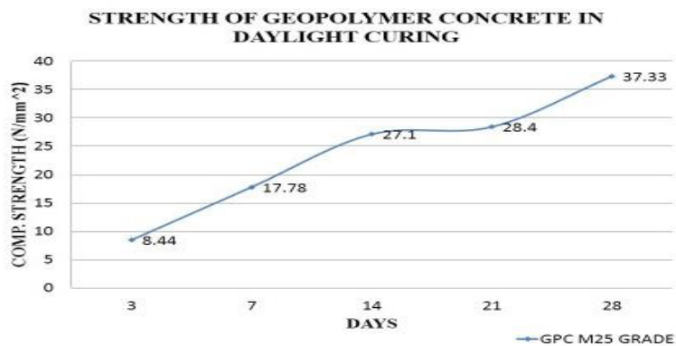
Fig. 1: The Compressive Strength of Geopolymer Concrete (12m)
