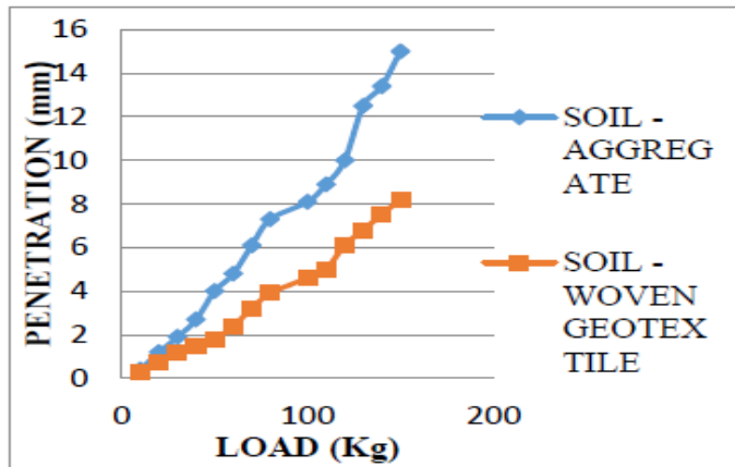
Figure 2. Soil-Woven-Aggregate
