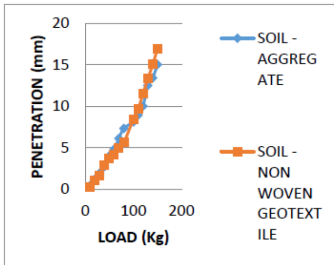
Figure 3. Soil-nonwoven-Aggregate
